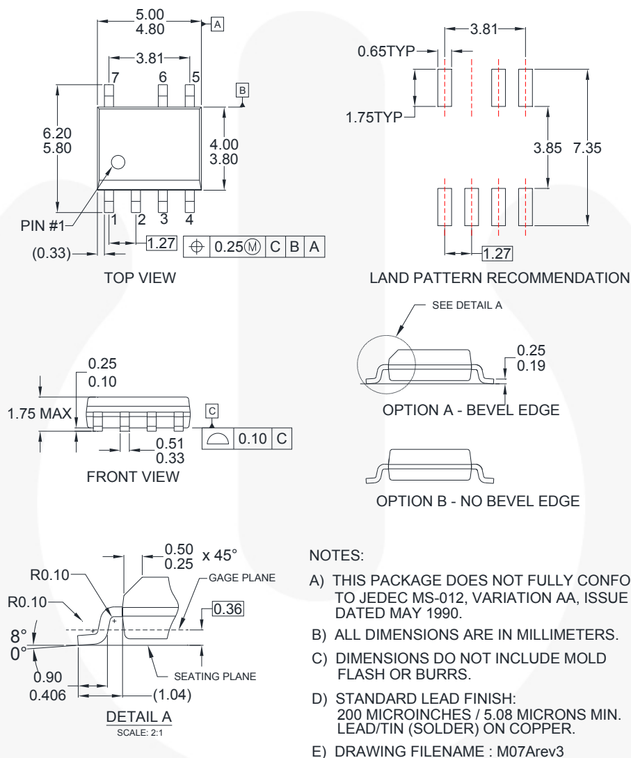
Figure 33. 7-Lead, Small-Outline Integrated Circuit Package (SOIC)
