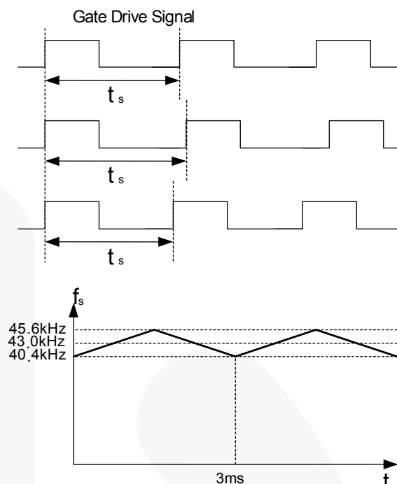
Figure 27. Frequency Hopping
