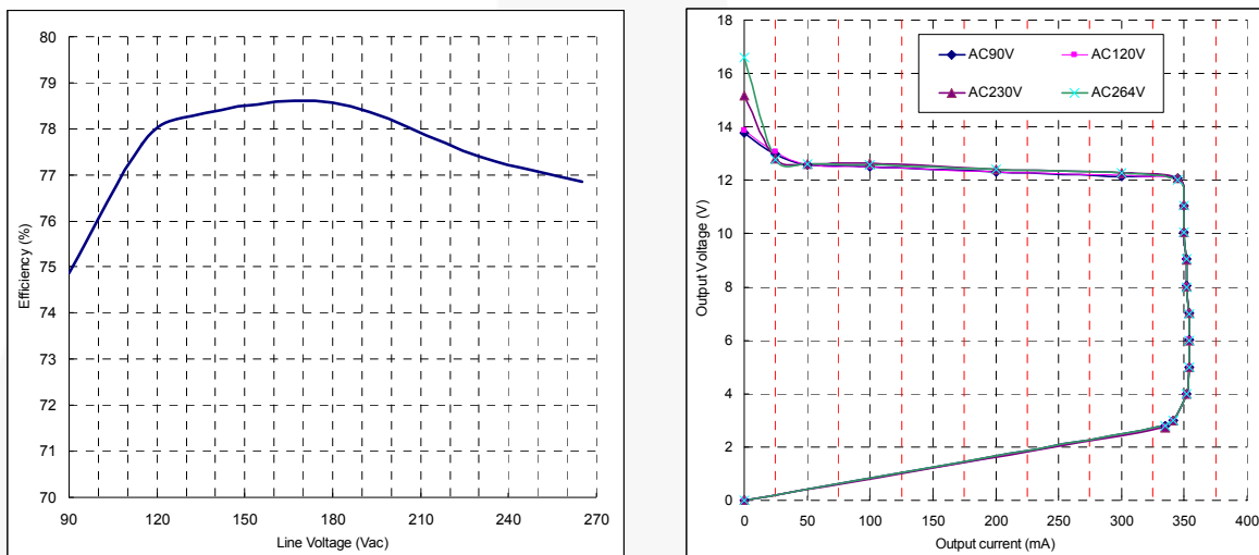
Figure 30. Measured Efficiency and Output Regulation
