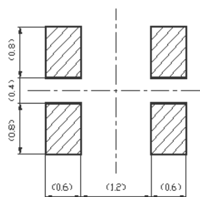
Land Pattern (Recommended)
