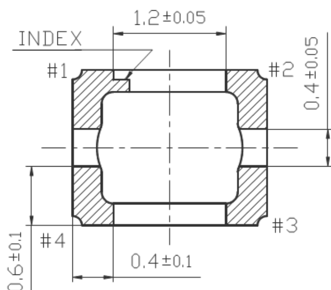
Land Pattern (Recommended)
