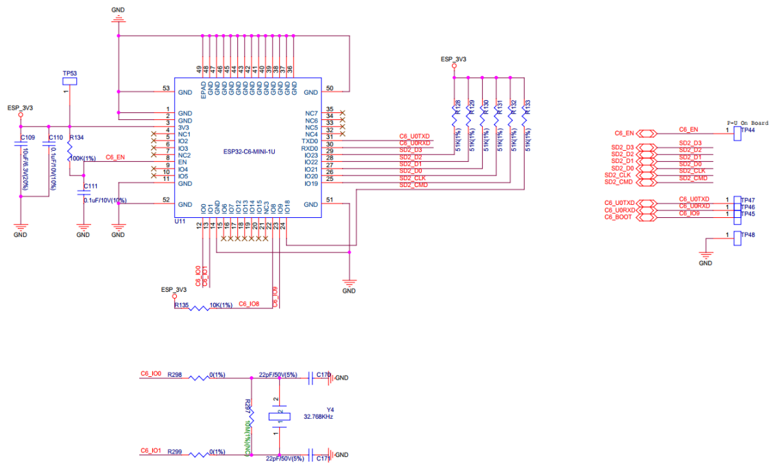
Fig. 17: ESP32-C6-MINI-1U Module Circuit (click to enlarge)
