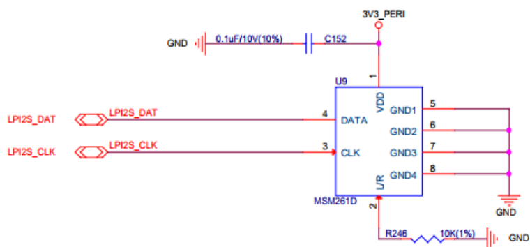
Fig. 14: Microphone Circuit (click to enlarge)
